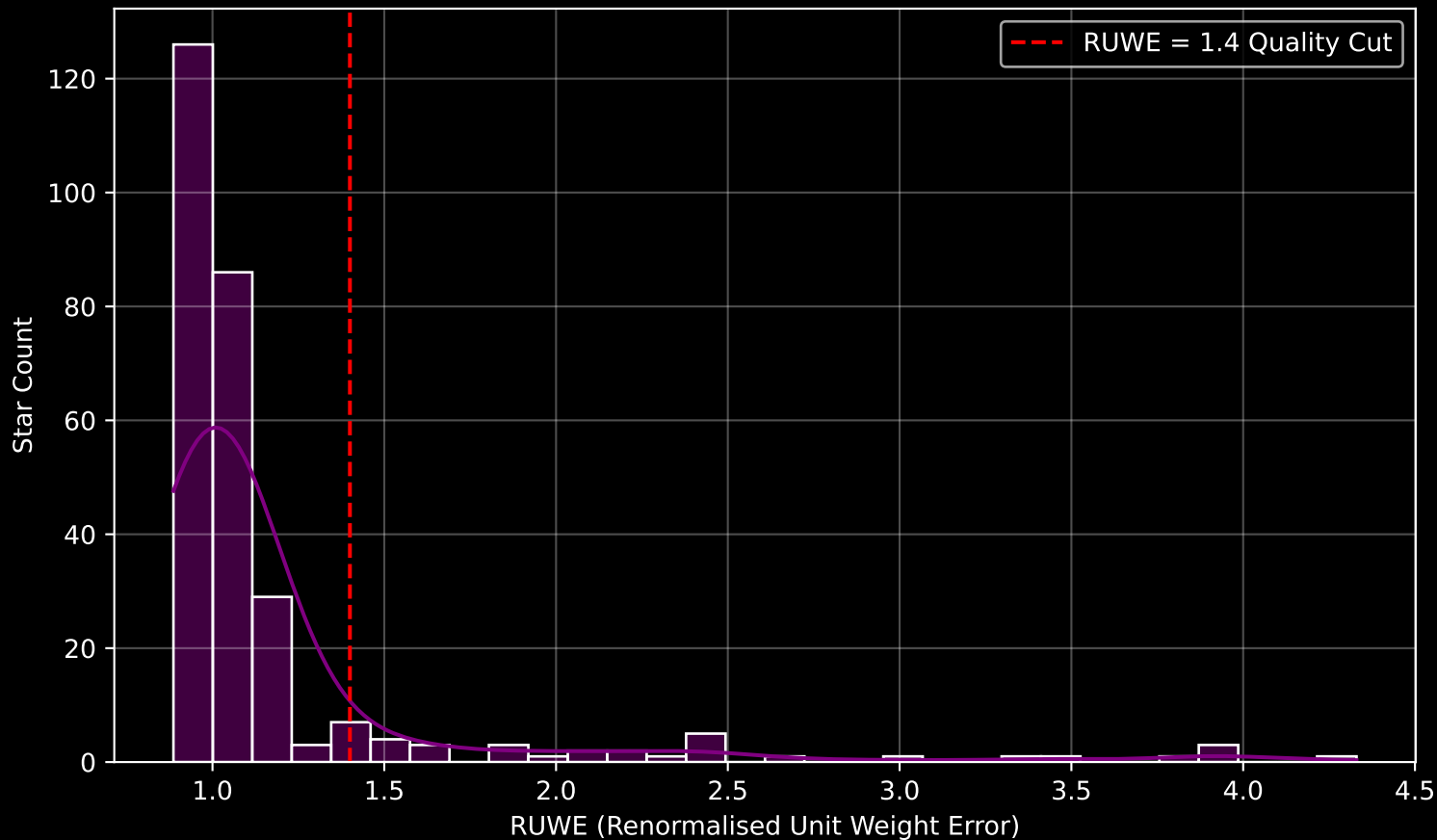
GALAH DR4 Field [728] RUWE Distribution (n= 281)
