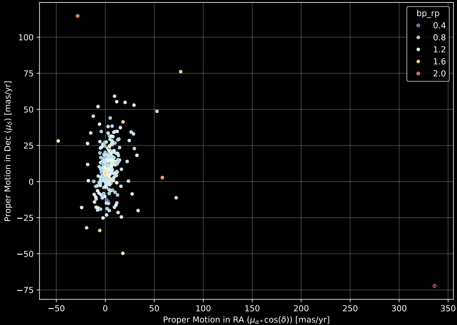
GALAH DR4 Field: [728] Proper Motion Diagram (n= 292)
