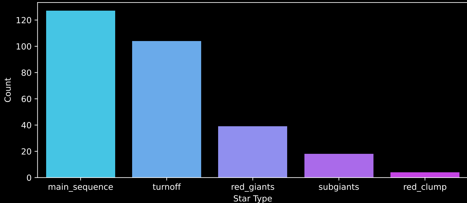
GALAH DR4 Field: [728] Count plot of Star Type
